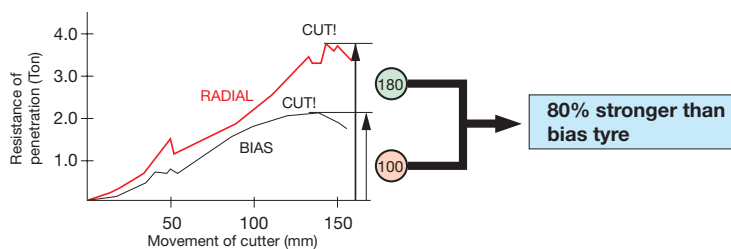
Force needed for object to penetrate the tyre
